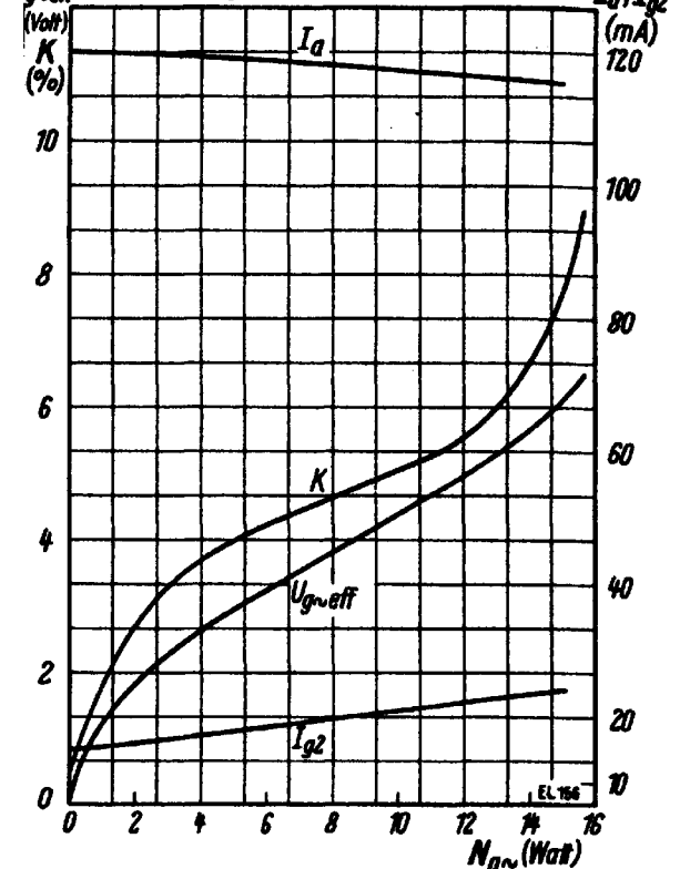
Kennlinienfeld 5 I_a, I_{g2}, U_{g\text{neff}}, K = f(N_{a\sim}) U_a = 350 \text{ Volt}, U_{g2} = 250 \text{ Volt}, R_a = 4 \text{ k}\Omega, R_k = 60 \Omega
